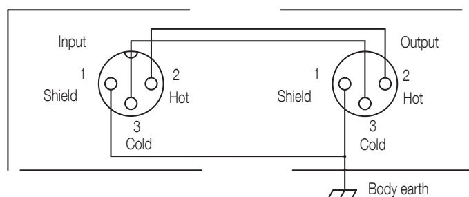
Circuit diagram
