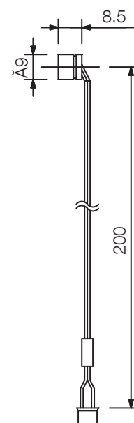
Hands-free microphone (accessory)
