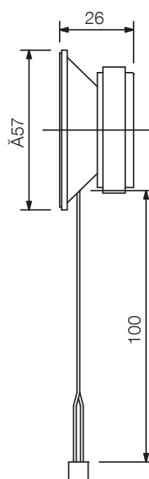
Hands-free speaker (accessory)
