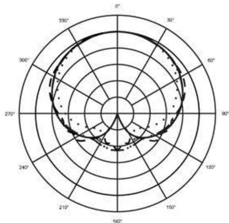
Polar Pattern
