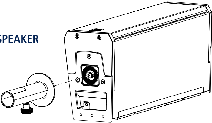
Pole Mount Kit for KX 515
