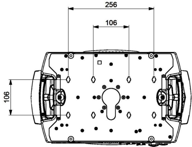
Quarter-turn receptacles in base
