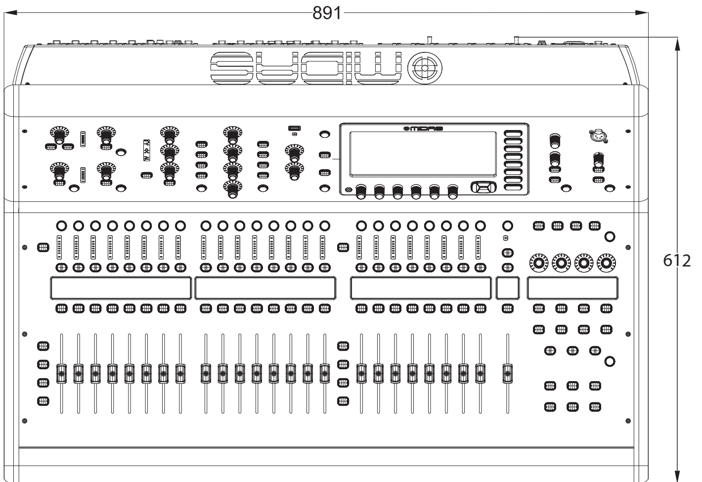
Top View
