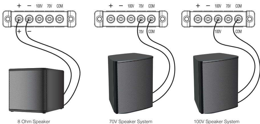
Figure 2.5.1 Output Wiring
