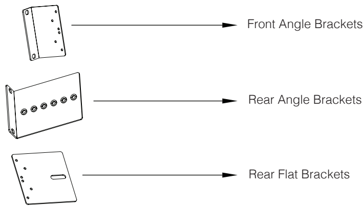
Figure 2.2.2 Mounting Kit
