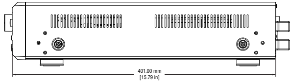
Figure 2.2.1 Dimensions
