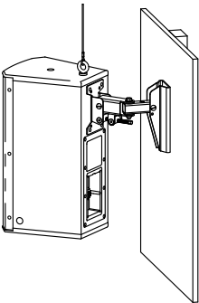
Figure 4.2: EVC-WB multi mount wall bracket
