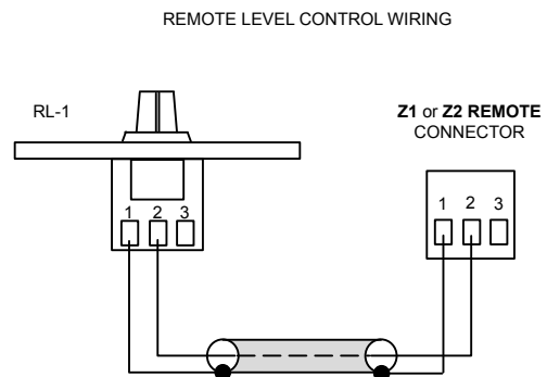
SINGLE-CORE SCREENED CABLE MAY BE USED
