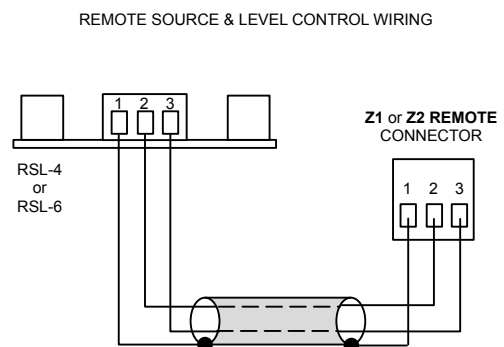
USE TWO-CORE SCREENED CABLE
