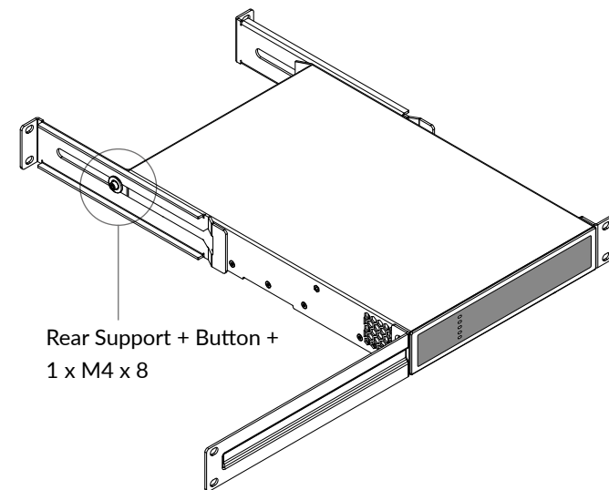
Diagram 4B CXA Rack Support hardware. 2 positions.
