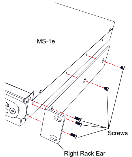
Rack Ear Installation
